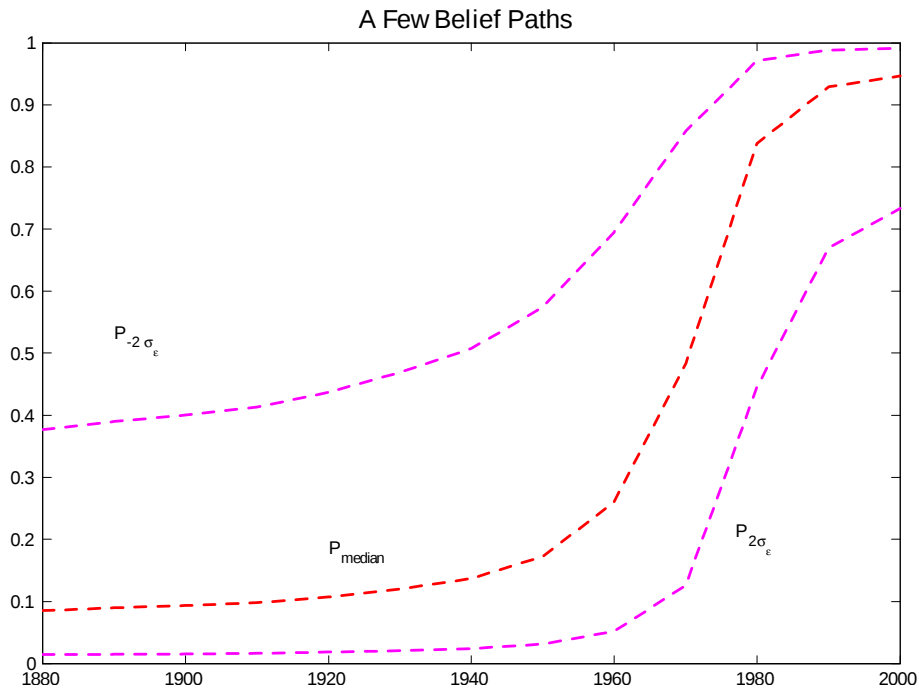
Figure 10: This shows \Pr(\beta^* = \beta_L) for agents with s = \beta^* and s = \beta^* \pm 2\sigma_\varepsilon .
