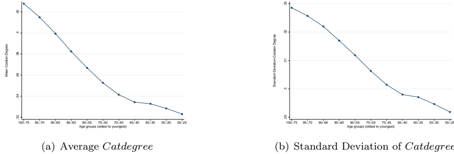
Figure 6: Evolution of CatalanDegree over (a moving window of) cohorts. Complete Population.
